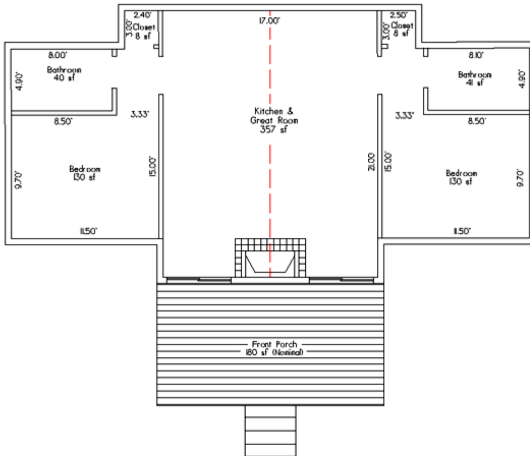
Existing Two Bedroom Unit
